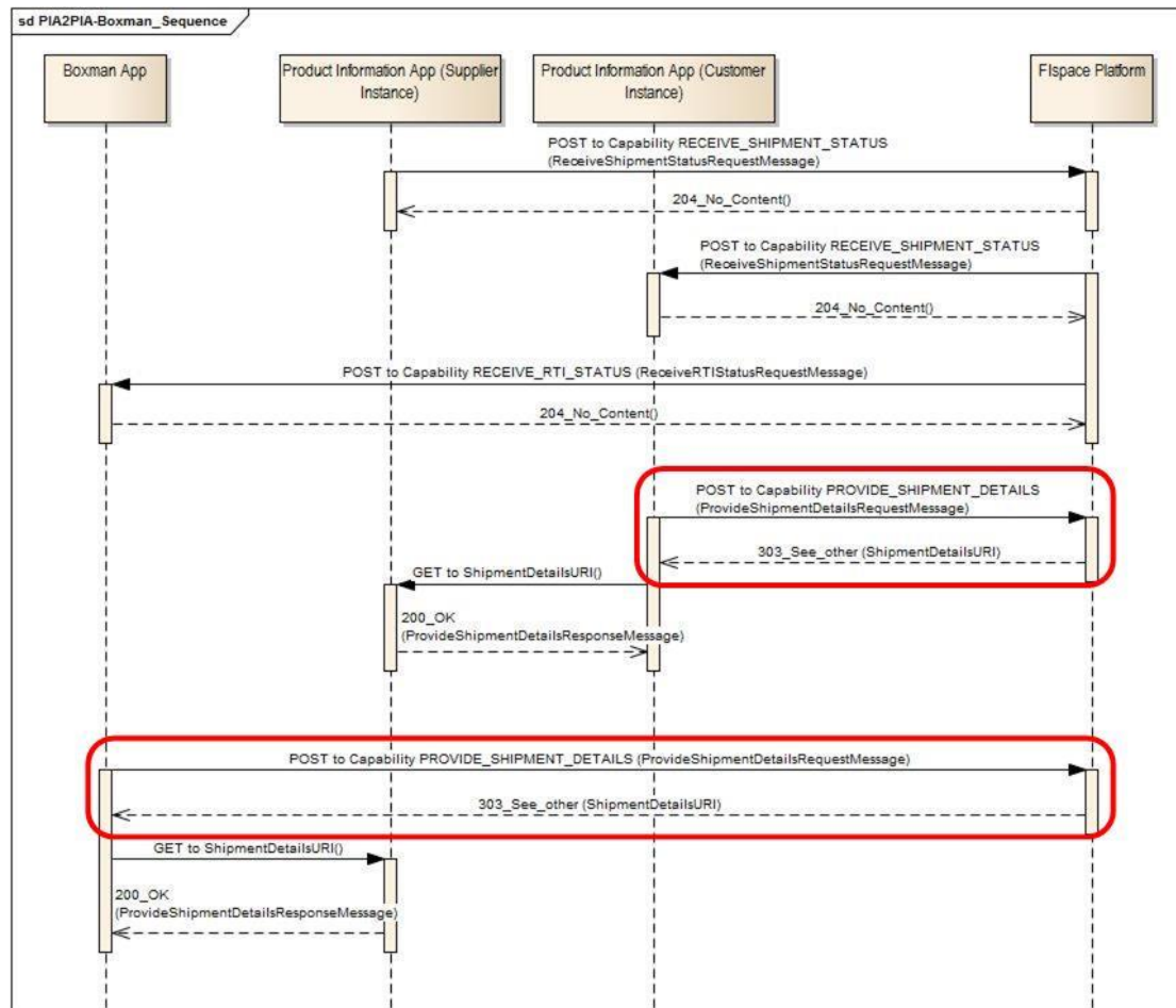
Figure 2. Workflow of two PIA instances and the BOXMAN app (with an abstract view on the FIspace platform)
