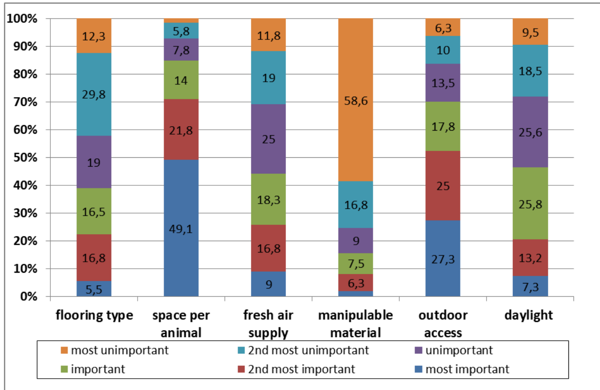
Figure 1. Ranking of stable-based aspects for fattening pig production 5 Source: own calculation and illustration
